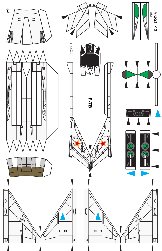
US Air Force Chengdu F-7B 4477th TES, 1980ies, Tonopah (NV)
